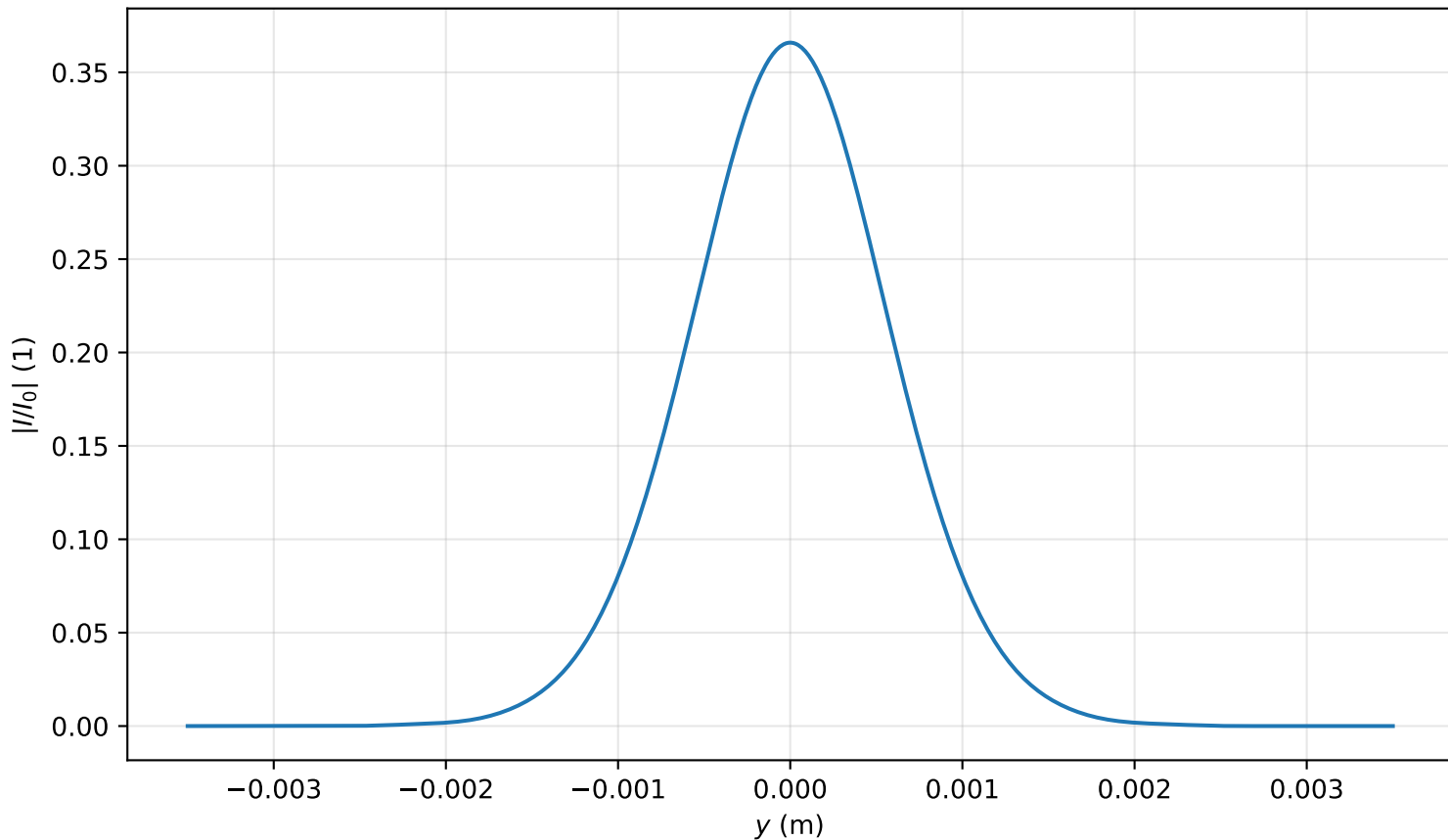
Intensity profile I(x=0, y, z=3.344)/I_0 , P_{in}=0.3P_{cr} , artificial time
